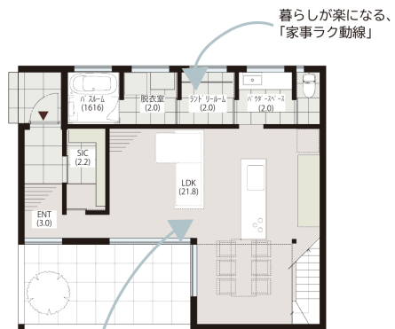
1st floor
